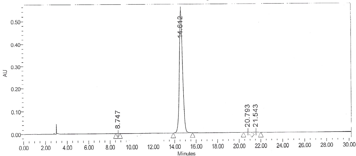
Auto-Scaled Chromatogram
